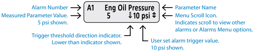
Figure 1-13: Viewing Alarms
