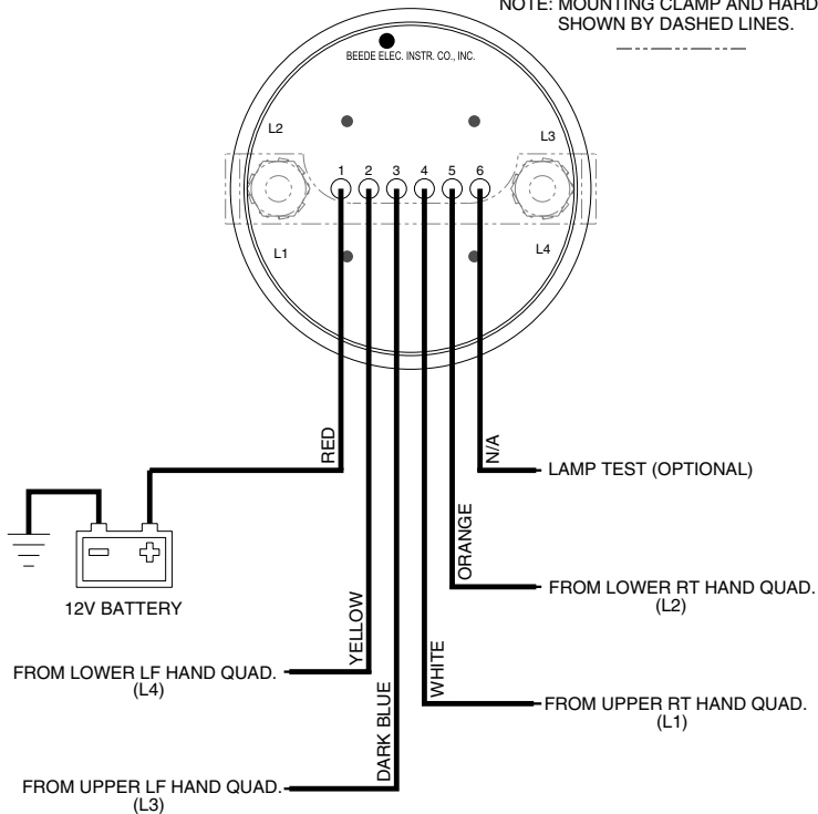
WARNING GAUGE (REAR VIEW)
